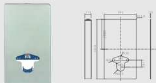
ECC887W WATER TANK ( For wall hung toilet )
