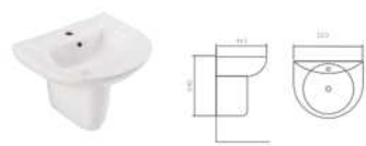
EB513W WALL HUNG BASIN
