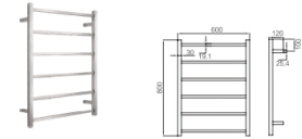
HTR800x600-6 Heater Towel Rail
